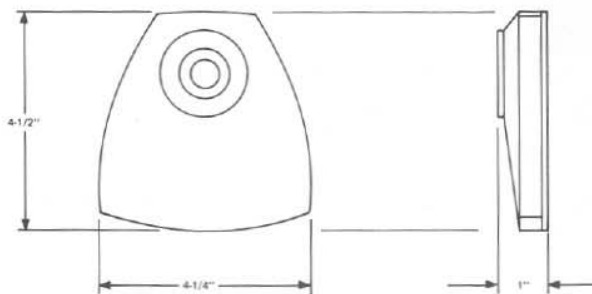
Figure 2 – Dimensions, model 422
