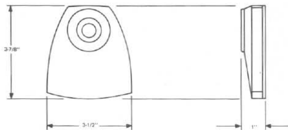
Figure 1 – Dimensions, model 421
